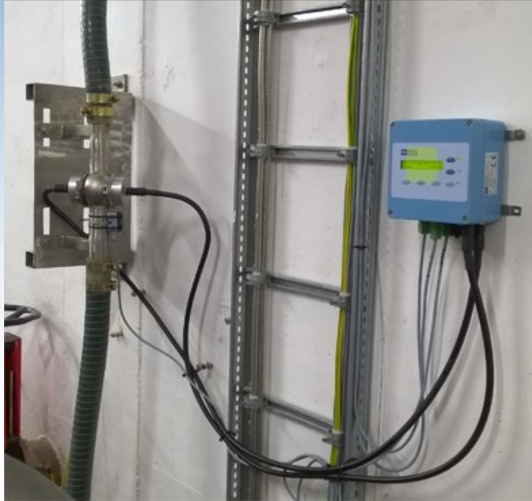
HK2 spiral antennas and PT100 Sludge
